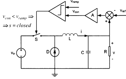
Fig. 1. The voltage mode controlled buck dc-dc converter.
