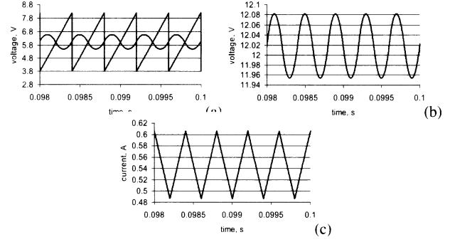
Fig. 2. The nominal period-1 operation of the buck converter: (a) the control and ramp signals, (b) the output voltage, and (c) the output current. The parameter values are V_{in} = 24V , V_{ref} = 11.3V , L = 20mH , R = 22\Omega , C = 47\mu F , A = 8.4 , T = 1/2500s , the ramp signal varies from 3.8V to 8.2V.
